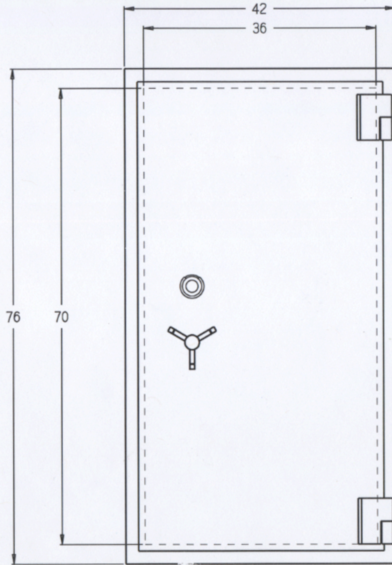
FRONT VIEW
